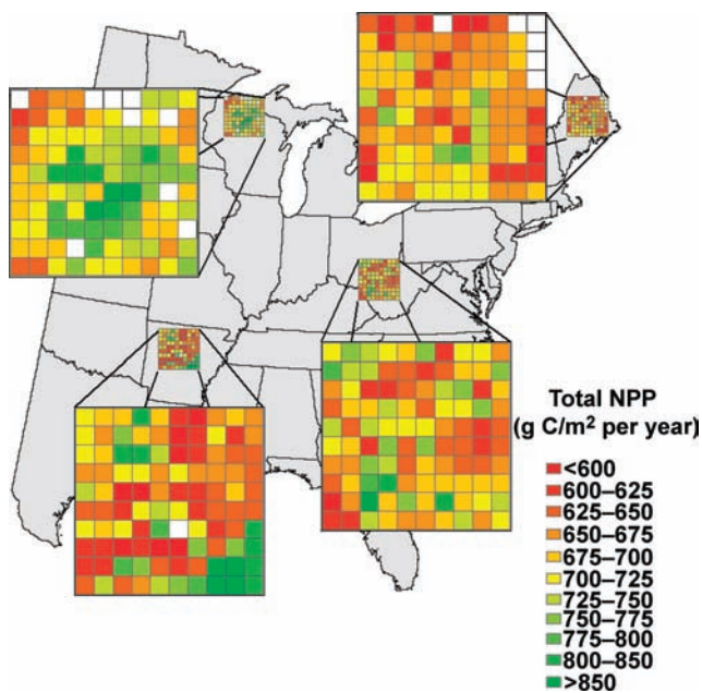
Figure 1. Net primary productivity (NPP) of forested area in each 20 × 20 km cell under the current climate. Sixteen cells (blank color fill) were excluded for the simulation due to the lack of data (e.g. outside the US border) or the coverage of water bodies.
