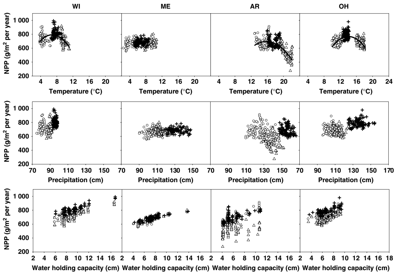
Figure 4. Sensitivity analysis of annual mean temperature, precipitation, and water-holding capacity on the responses of annual net primary productivity (NPP). Under current ( \circ ), HAD2CM ( \Delta ), and CCC (+) climatic scenarios, NPP of combined species and climatic change effects were used for the analysis. Annual mean temperature and precipitation of each 20 \times 20 km cell varied with climatic scenarios while water-holding capacity was kept constant for each individual cell. See Table 2 for the statistical results and the polynomial curve fitting of the relationships between NPP and temperature in Wisconsin (WI), Arkansas (AR) and Ohio (OH).
