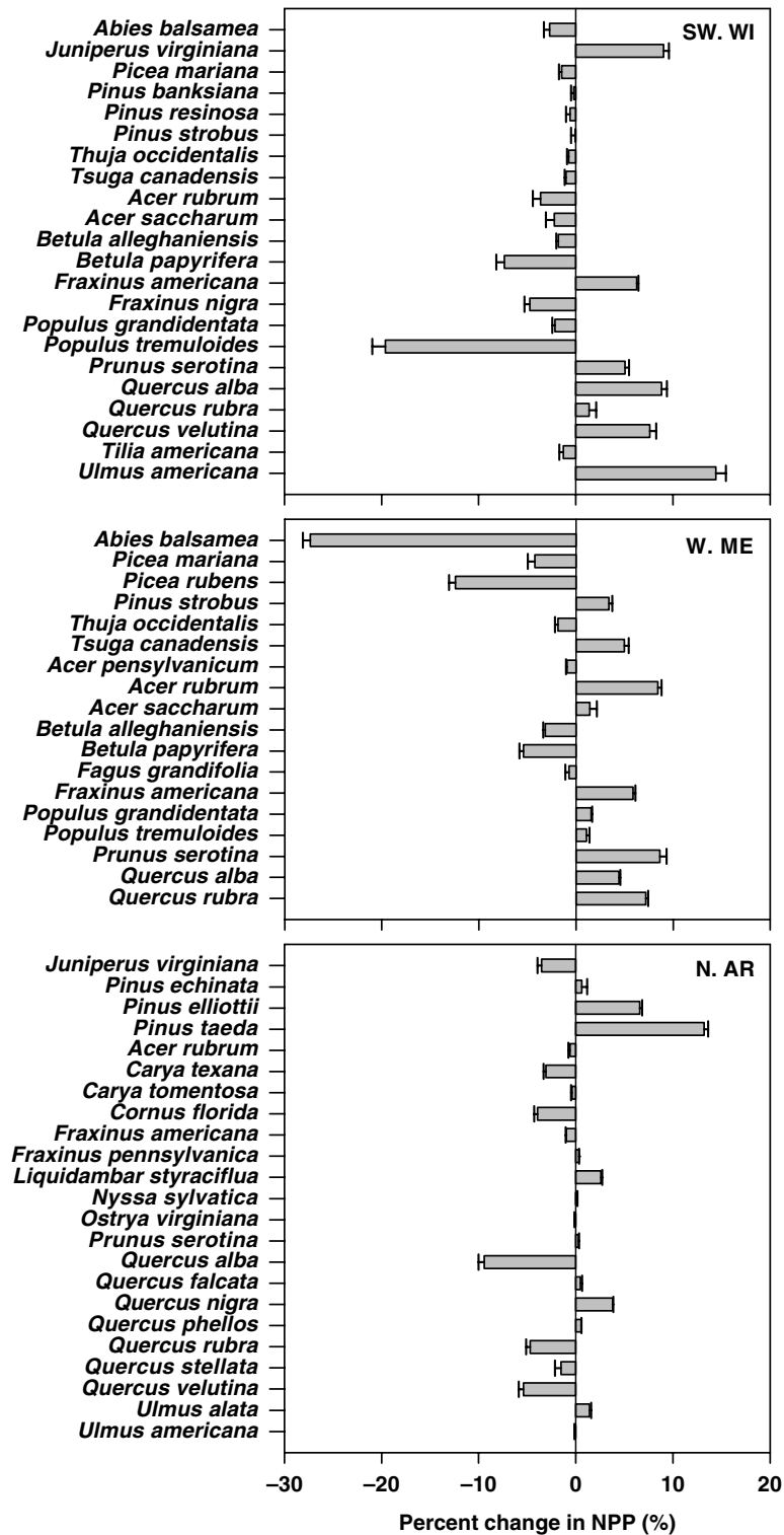
Figure 3. The net effect of species-specific changes in the abundance on net primary productivity (NPP) of areas where substantial species effects on NPP were predicted under CCC climatic scenario. The areas include northern Arkansas (49 cells; < 2% NPP change), southwestern Wisconsin (13 cells; > 2% NPP change), and western Maine (24 cells; < 6% NPP change).
