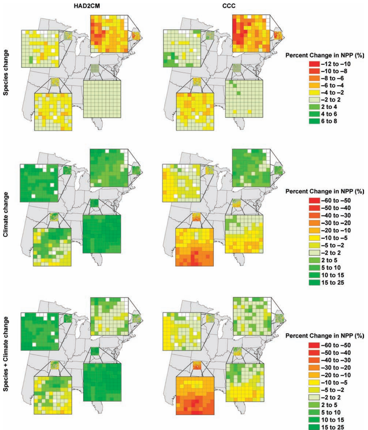
Figure 2. Percent changes of annual net primary productivity (NPP) due to the effects of species range shift, climate change and the combination of both. HAD2CM and CCC are climatic scenarios, under which the effects of resulting species range shifts, climate change, and the combination of both on NPP were simulated. Due to the much narrower range of variations, the color ramp for species change effects was different from the other two effects.
