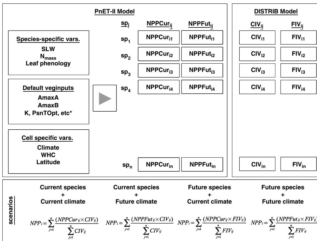
Figure 5. The merging of PnET-II (forest carbon balance model) and DISTRIB (forest species composition model) models. A_{maxA} , intercept of the relationship between foliar nitrogen content and maximum photosynthetic rate; A_{maxB} , slope of the relationship between foliar nitrogen content and maximum photosynthetic rate; CIV_{ij} , the relative importance value of the i th cell for the j th species under the current climate; FIV_{ij} , the relative importance value of the i th cell for the j th species under the future climatic scenarios; K, canopy light attenuation constant; N_{mass} , leaf nitrogen content (% mass); NPP_{Cur_{ij}} , net primary productivity of the i th cell ( 20 \times 20 km cell) for j th species under the current climate; NPP_{Fut_{ij}} , net primary productivity of the i th cell for the j th species under the future climatic scenarios (HAD2CM or CCC); PsnTOpt, optimum temperature for photosynthesis ( ^{\circ}C ); SLW , specific leaf weight ( g/m^2 ); vars., variables; WHC, water holding capacity (cm). *Other default parameter inputs are listed in Aber et al. (1995).
