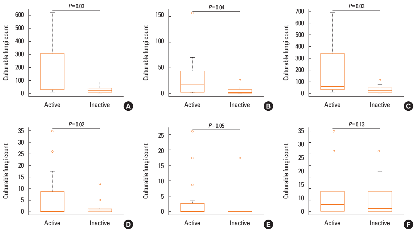
Fig. 2. The Box-and-Whisker plot of fungal spore concentration (CFU/m 3 ) in the active and inactive stages among patients with positive ImmunoCAP test results for specific IgE to the designated fungal allergens. (A) Cladosporium oxysporum , (B) Cladosporium cladosporioides , (C) Cladosporium spp., (D) Aspergillus niger , (E) Penicillium brevicompactum , and (F) Penicillium oxalicum .
