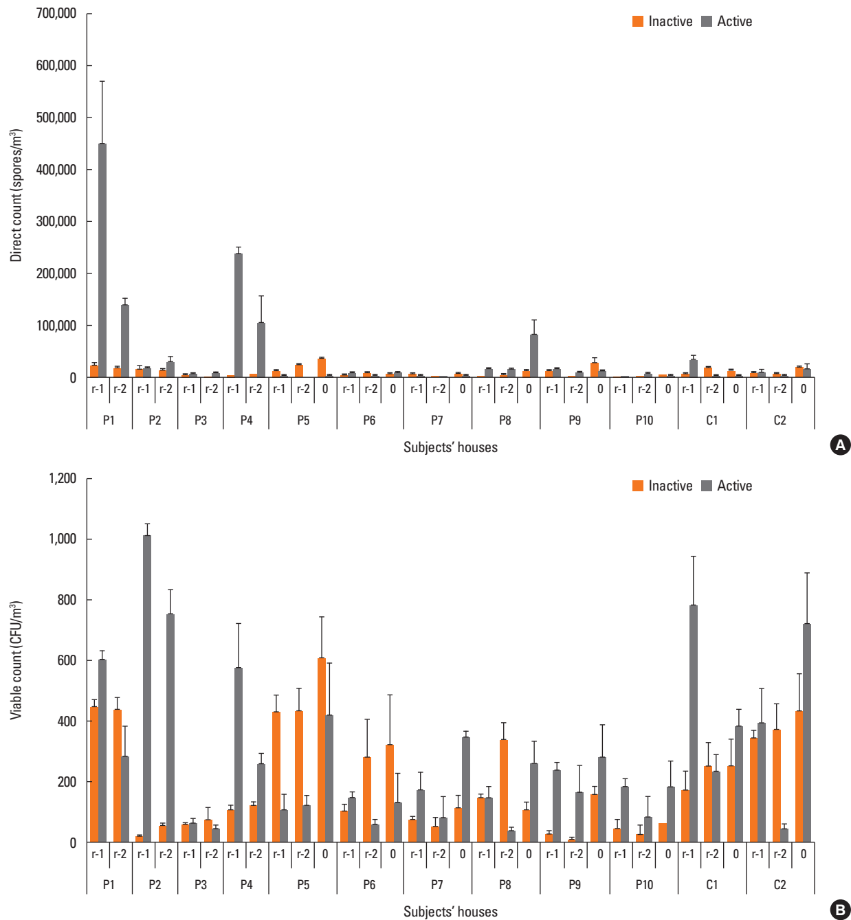
Fig. 1. (A) Direct spore count in the subjects' houses during the active and inactive stages of allergy, (B) Viable count in the subjects' houses during the active and inactive stages of allergy. r-1 and r-2 denote mean spore counts in room 1 and room 2 for each patient. 0 denotes means of outdoor spore counts for each patient.
