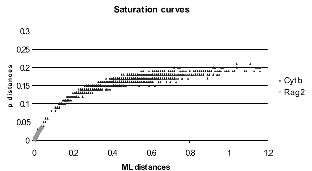
Fig. 1. Uncorrected (p-distance) pairwise distances plotted against ML distance (corrected with GTR + \Gamma_8 + I) measured for the Cyt b (black triangle) and Rag 2 (light grey cross) datasets. This saturation curve indicates that Cyt b substitutions reached a plateau beyond about a p-distance of 0.15.
