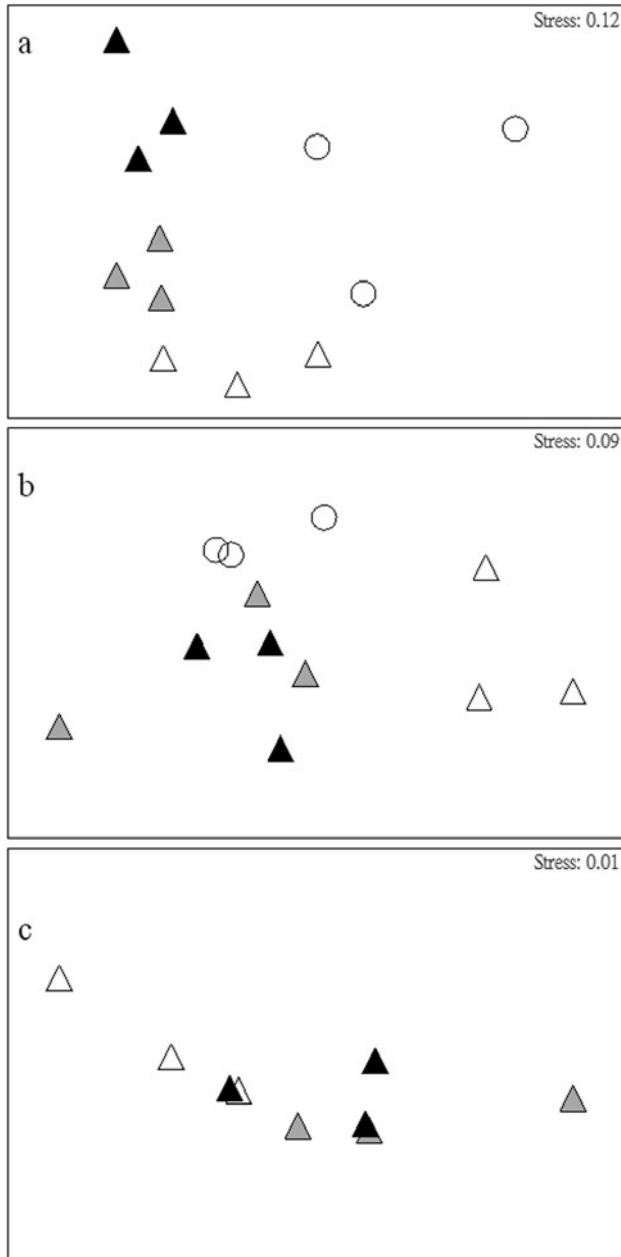
Fig. 2. MDS ordination of soil microbial communities and functions from the broadleaf forest and the unthinned, lightly thinned, and heavily thinned plantation forests. a. soil fungal communities from DGGE profiles; b. soil bacterial communities from DGGE profiles; c. soil functions from Biolog assay. White circle (○), broadleaf forest; white triangle (△), unthinned plantation forest; gray triangle (▲), lightly thinned plantation forest; black triangle (▲), heavily thinned plantation forest.
